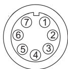
7 pin female connector - pinout external view
