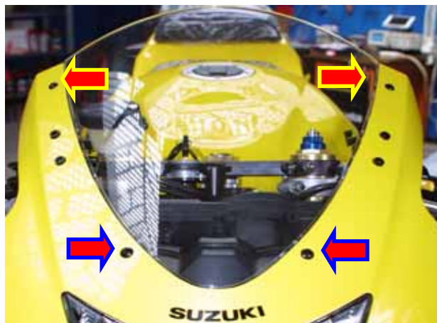
Figura 3: Cupolino – 4 viti autofilettanti Phillips.
