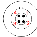
4 PIN FEM. BINDER CONNECTOR PINOUT
