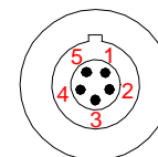
5 PIN FEM. BINDER CONNECTOR PINOUT
