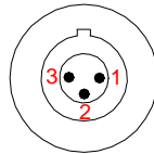
3 PIN FEM. BINDER CONNECTOR PINOUT
